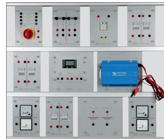
Set of photovoltaic modules (H-250mm) and solar panels for studying a solar installation on an isolated site.
