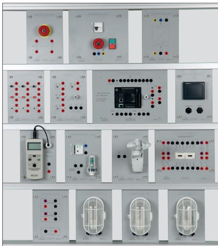
Sets of modules (H-250mm) and sensors for studying a PLC with touch screen
