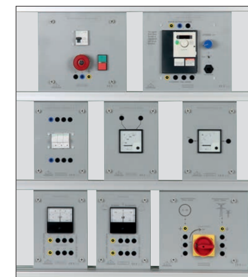
The set can be supplied without the motor set, without capacitive or resistive load, please ask for details.
